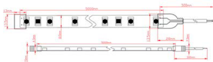
Product Dimensions (mm)
